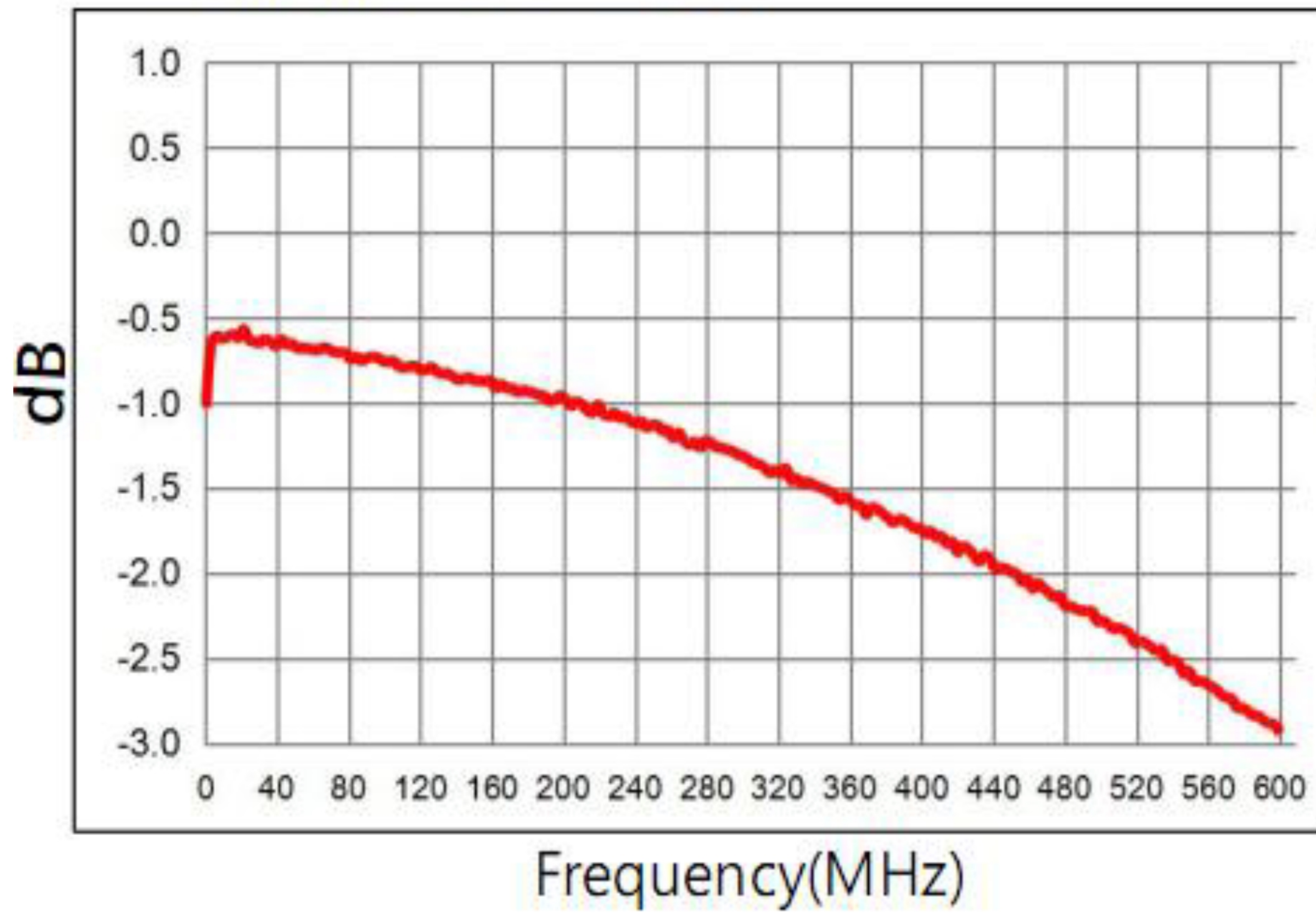
Main line Loss(out1)
