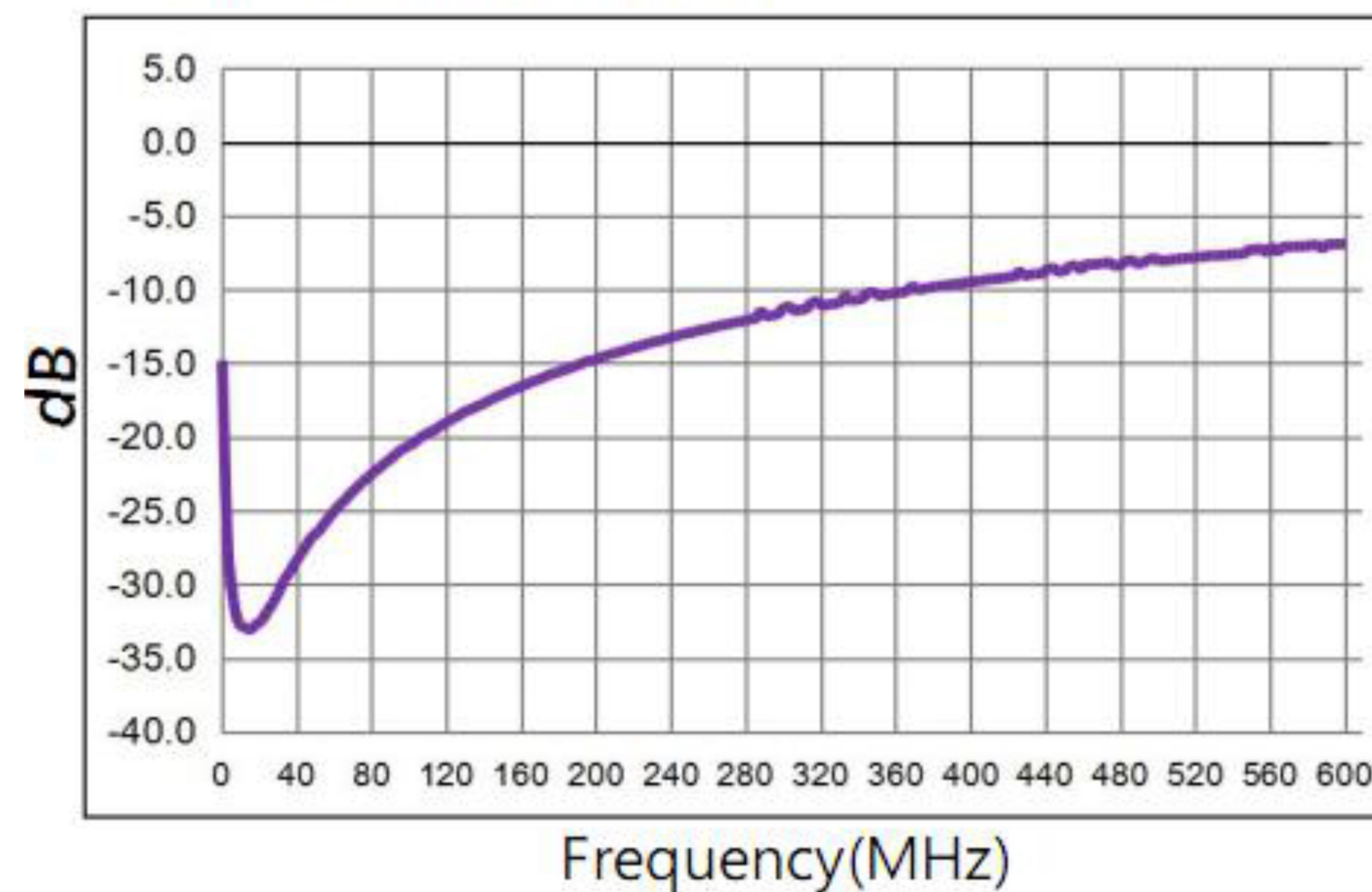
Input Return Loss
