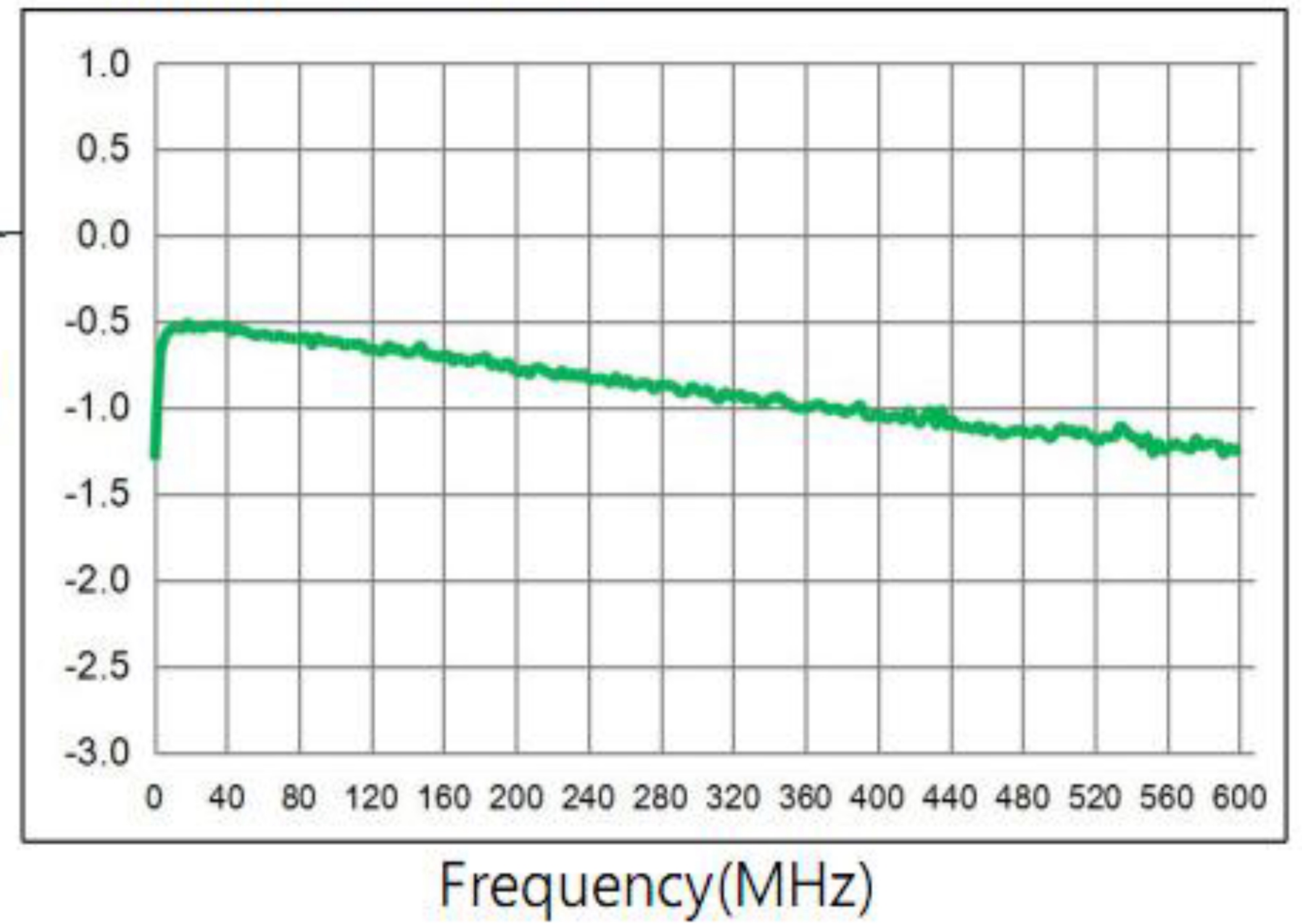
Main line Loss(out2)
