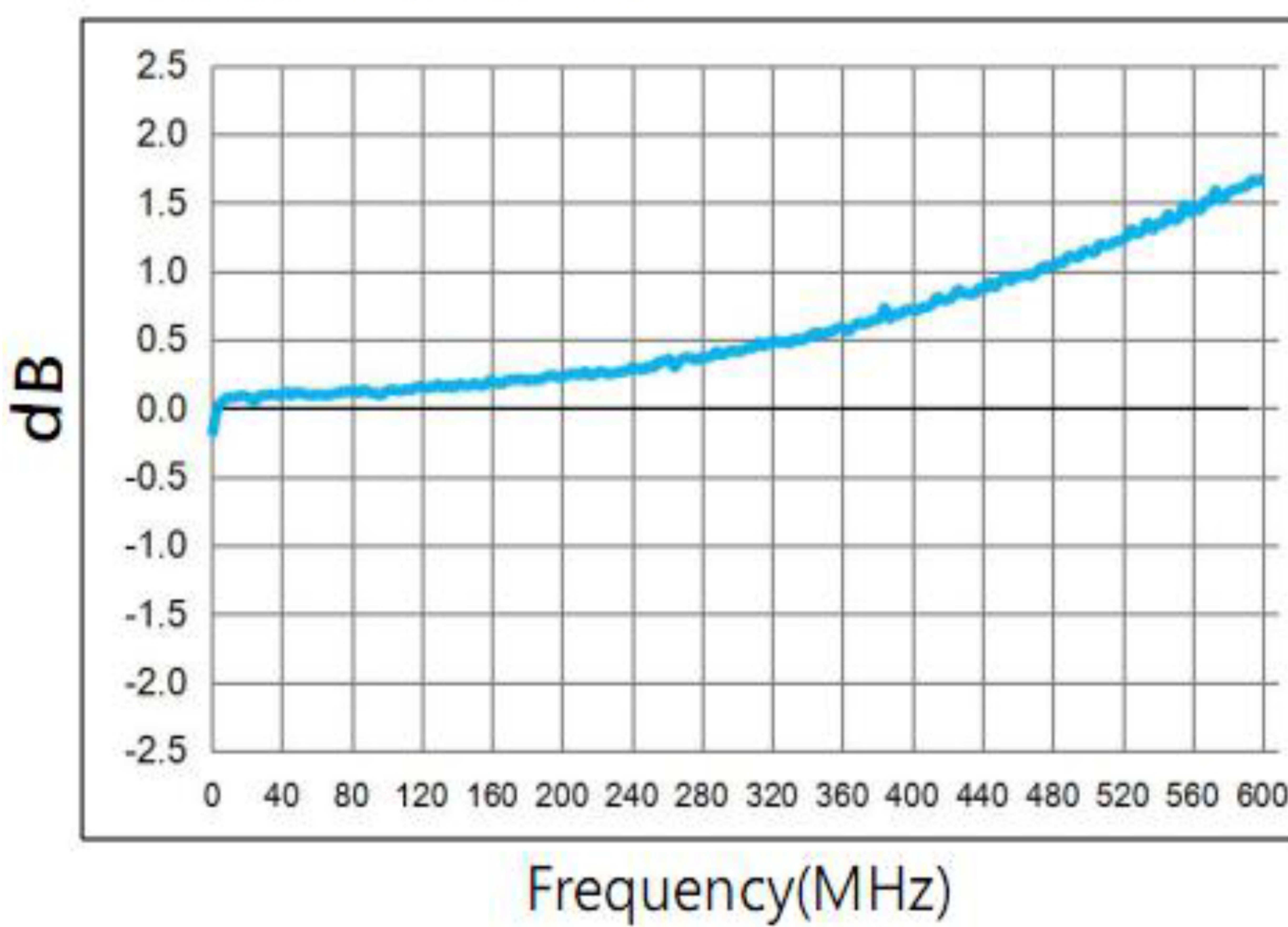
Amplitude Balance
