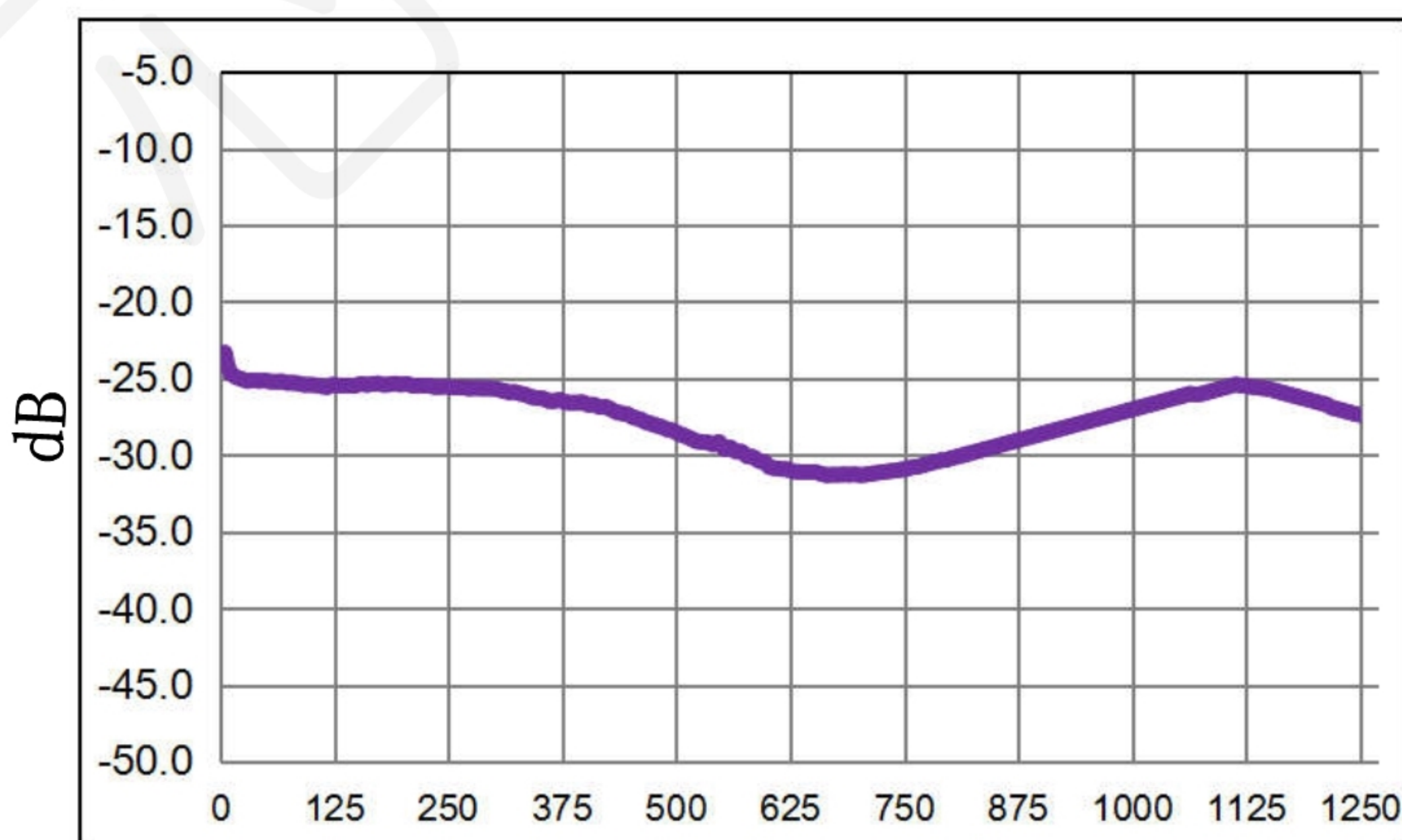
Input Return Loss
