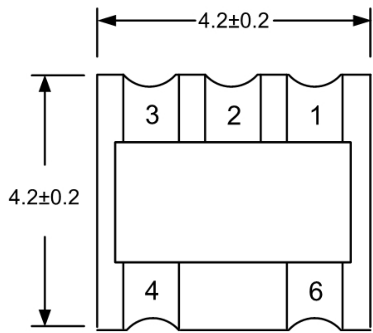
Top View
