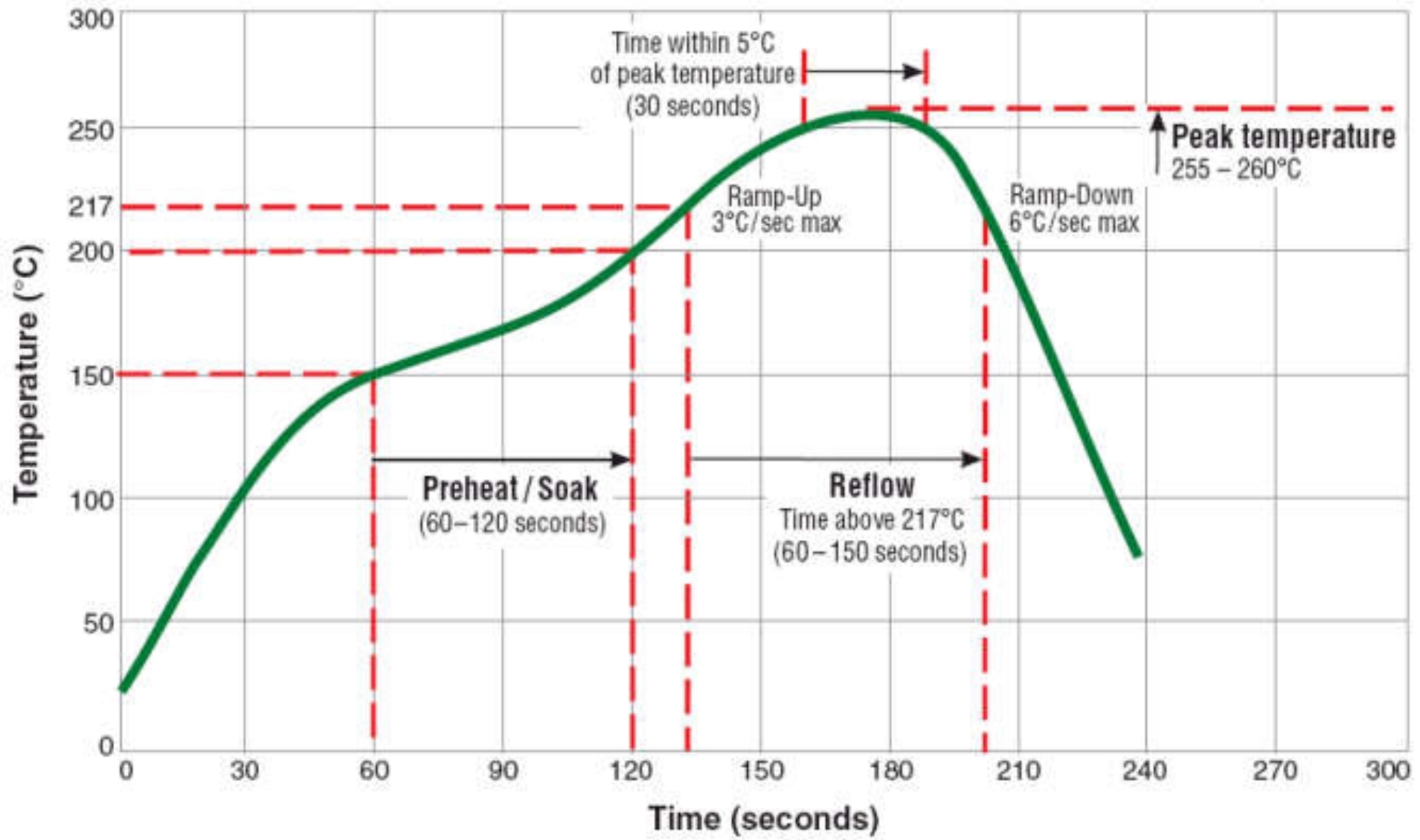
Typical RoHS Reflow Profile
